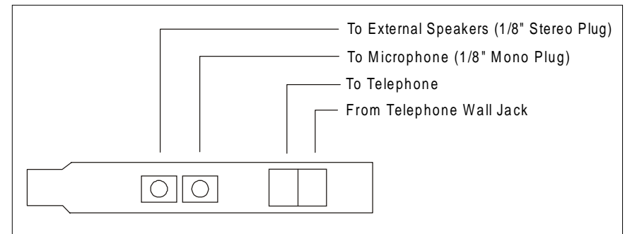
Fig. 2 Board Configuration
