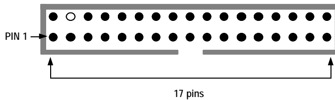
Top View of the Floppy Disk Drive Connector
