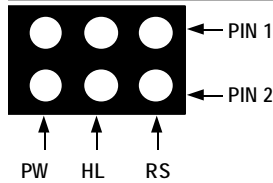
Top View of the System Panel Buttons and LED Connectors
