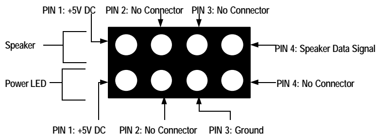
Top View of Speaker and Power LED Connector
