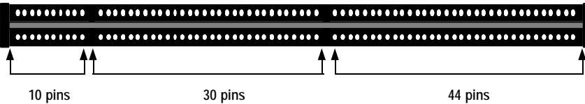
Top View of a 168-pin DIMM Socket
